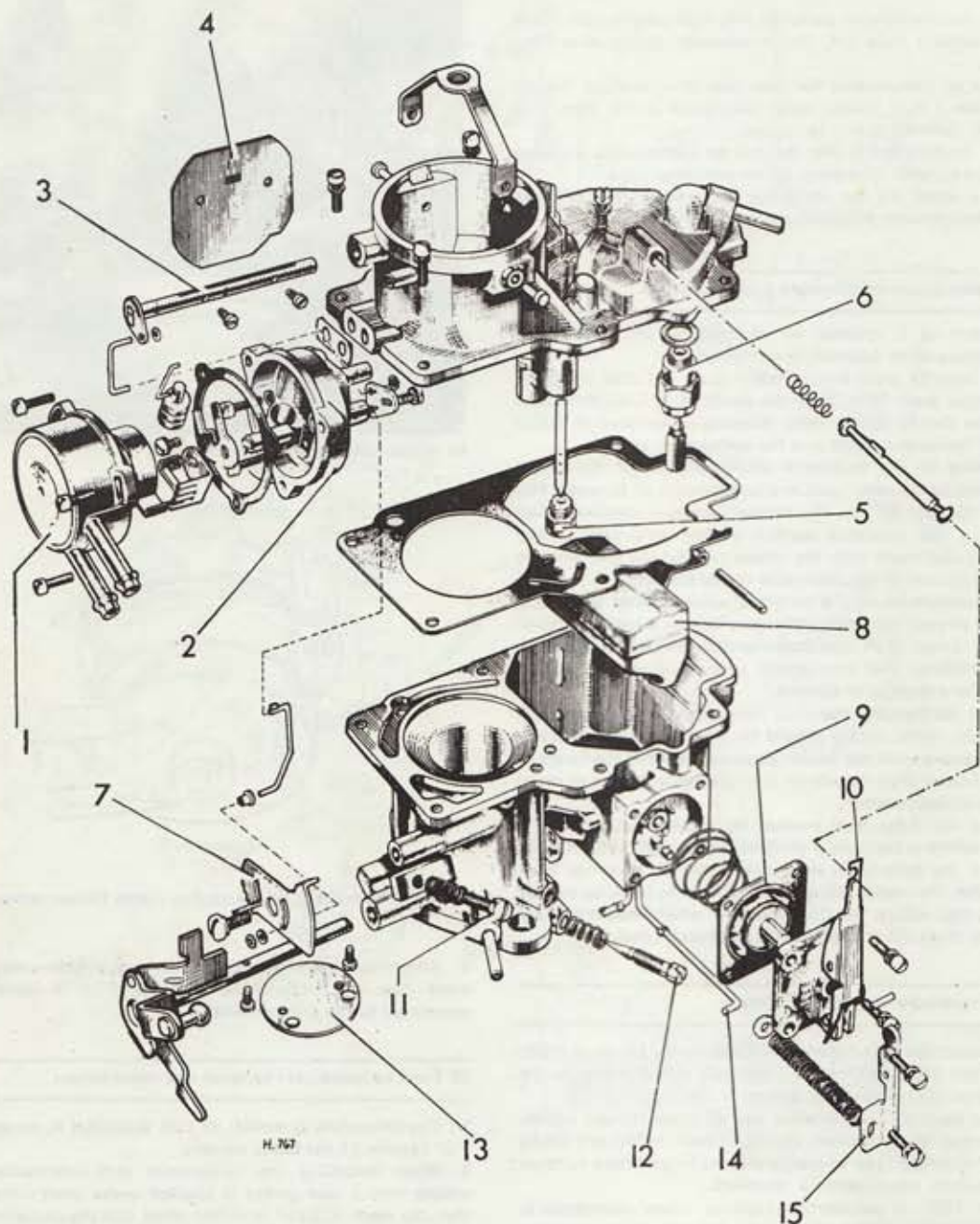
Fig 3.10 Exploded view of Ford type carburettor (1969-70)
